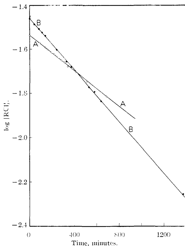
Fig. 1.—First-order ethanolyse of the isomeric 5-methyl-2-cyclohexenyl chlorides at 30°C: A, trans -isomer (IIb); B, cis -isomer (Ib).
